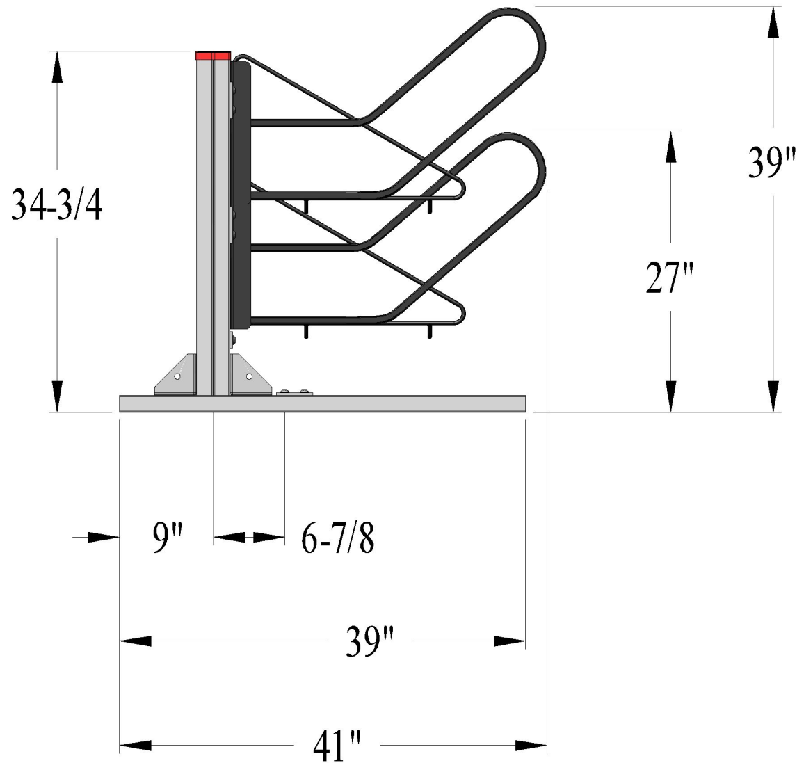
Bike Stall {8-Bike} U-Strut Strut Base {Straight} Assembly {Side} Dim's
