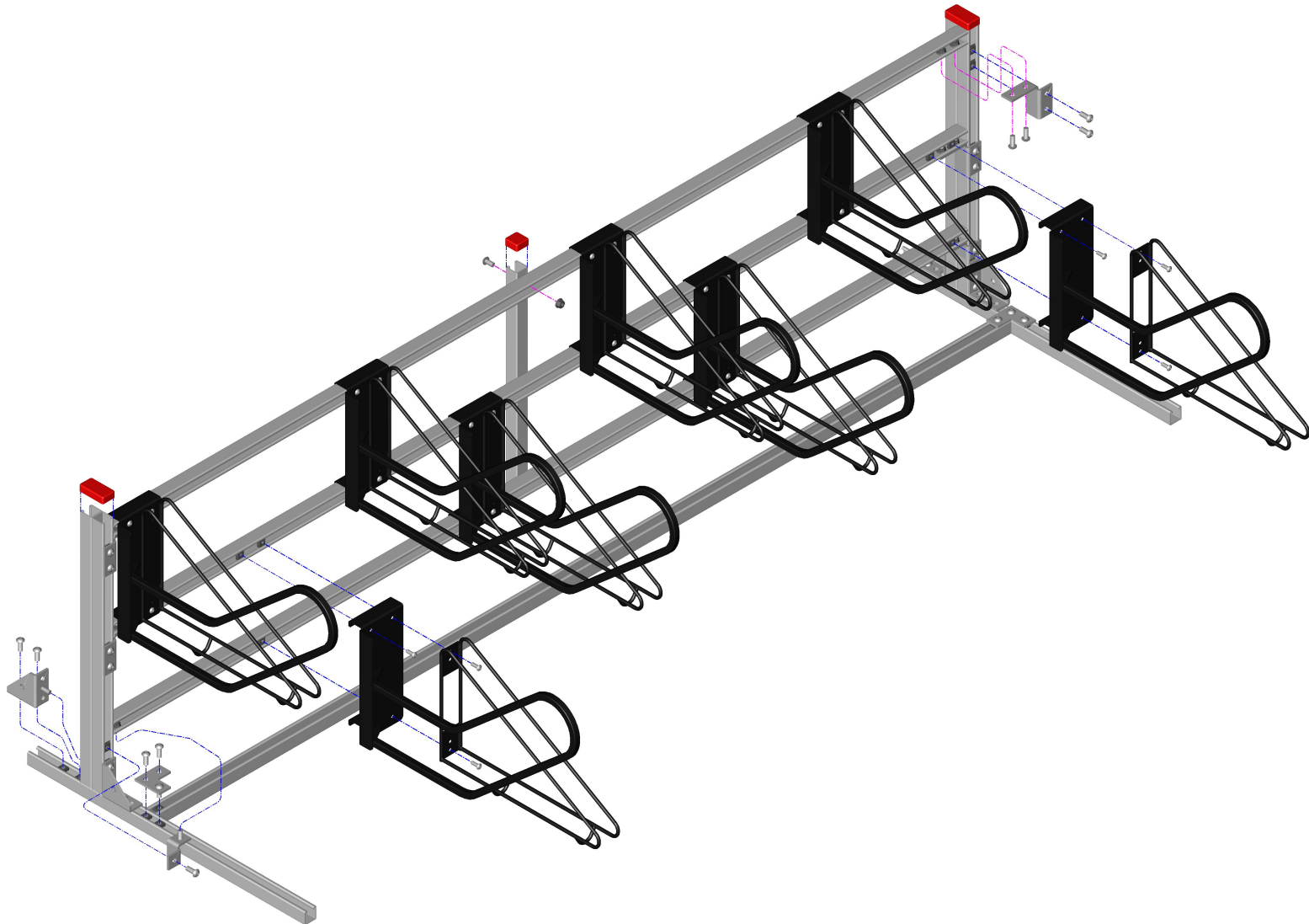
Bike Stall {8-Bike} U-Strut Strut Base {Straight} Assembly {Exploded}
