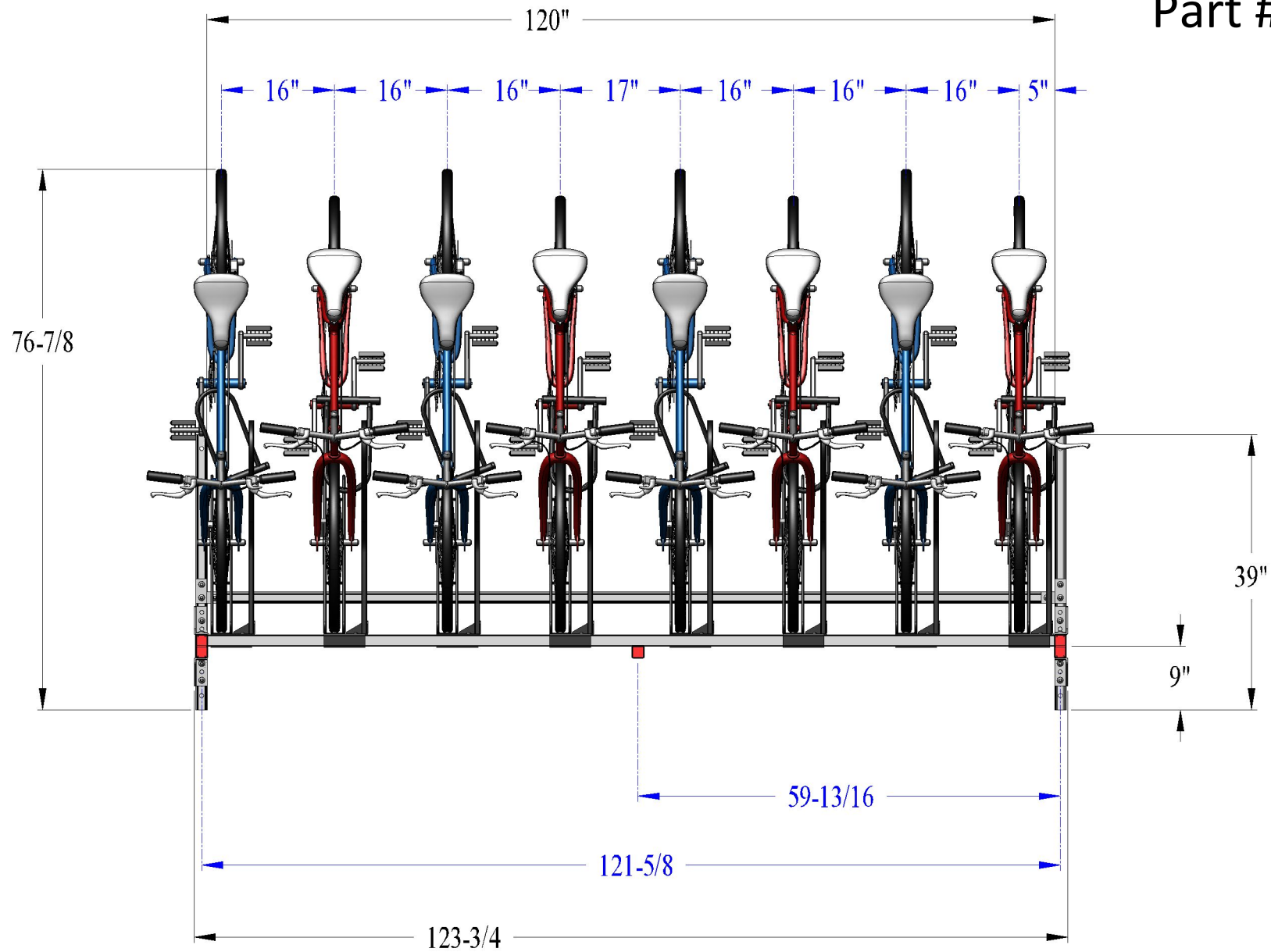
Bike Stall {8-Bike} U-Strut Strut Base {Straight} Master {Top} Dim's
