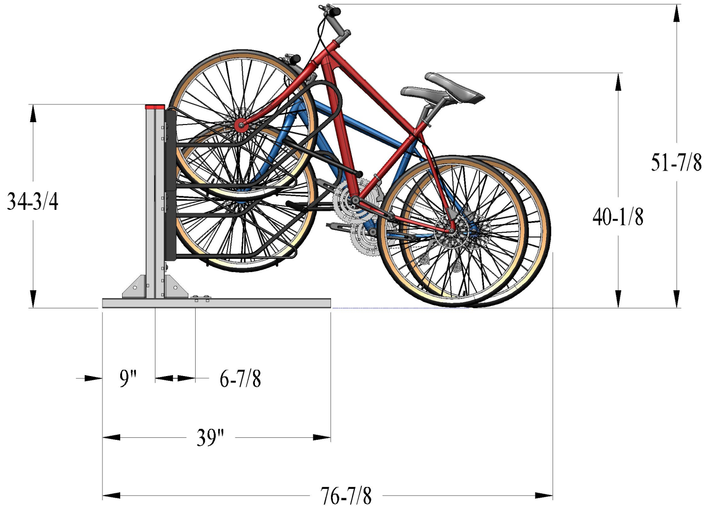
Bike Stall {8-Bike} U-Strut Strut Base {Straight} Master {Side} Dim's
